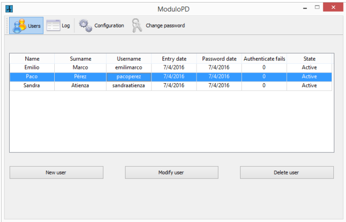
Fig. 2. Main window
